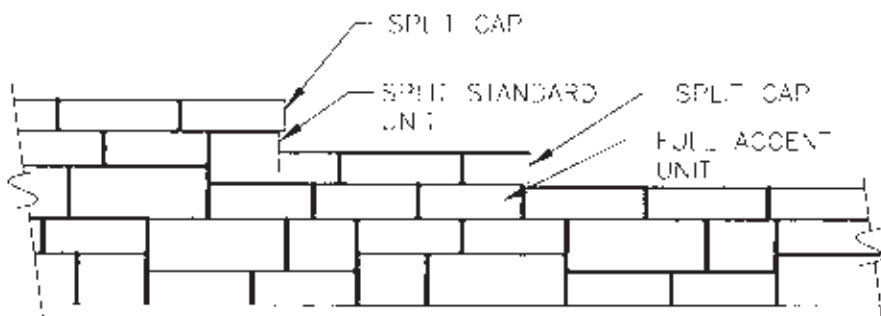
FIGURE 10 SPLIT UNIT DETAIL
