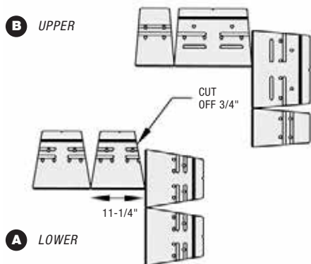
First Course
