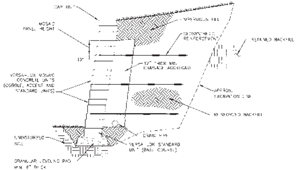
TYPICAL SECTION REINFORCED RETAINING WALL SCALE: NONE
