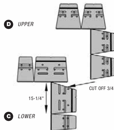
Second Course
